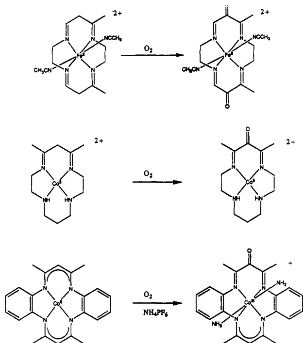
Figure 39. The autoxidation of the \gamma carbon to a carbonyl group in \beta -diimine chelate rings of iron(II) and cobalt(II) complexes.
