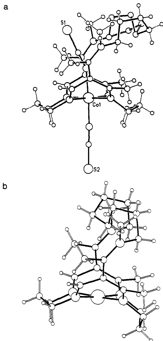
Figure 17. Cyclidenes with -(\text{CH}_2)_6- bridges: (a) the \text{Co}(\text{NCS})_2 complex, \text{Co}^{\text{III}}(\text{C8MeMe}[16]\text{Cyc})(\text{NCS})_2 ; (b) Cu complex without additional ligands, \text{Cu}^{\text{II}}(\text{C8MeMe}[16]\text{Cyc}) (cf. Figure 7b).
