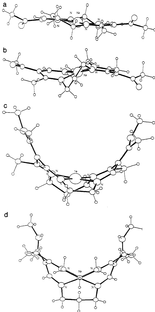
Figure 4. The effect of varying macrocycle ring size in unbridged cyclidene and related complexes (a) a [14] ring, \text{Ni}^{\text{II}}(\text{Ac}_2\text{HMe}[14]\text{Jag}) ; (b) a flat [15] ring, \text{Ni}^{\text{II}}(\text{Ac}_2\text{HMe}[15]\text{Jag}) ; (c) a buckled [15] ring, \text{Ni}^{\text{II}}(\text{Me}_2\text{Me}[15]\text{Mjg}) (252:3C) (d) a [16] ring, \text{Ni}^{\text{II}}(\text{Tca}_2\text{HMe}[16]\text{Jag}) .
