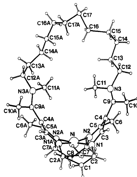
Figure 8. The -(\text{CH}_2)_{12}- bridged cyclidene complex \text{Ni}^{\text{II}}(\text{C12MeMe}[16]\text{Cyc}) , showing the lid-on conformation of the outermost nitrogen atoms (contrast Figure 7b).
