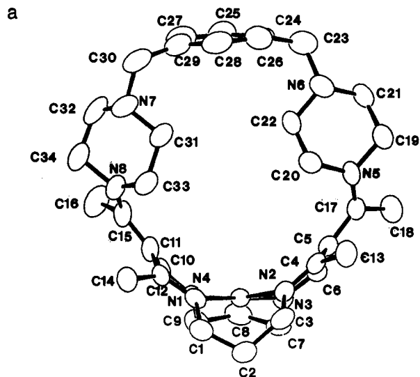
Figure 9. A p -xylylene-bridged cyclidene, Ni II ( p XyHMe[16]Cyc).
