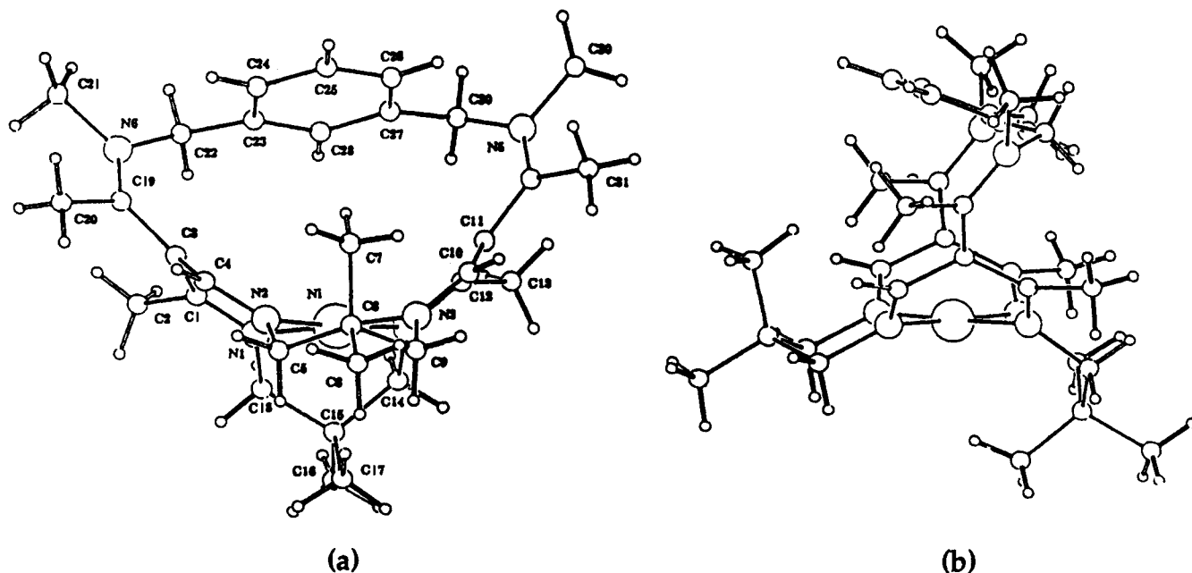
Figure 14. gem -Dimethyl substitution on both the X and Y rings, \text{Ni}^{\text{II}}(\text{mXyMeMe}[\text{Me}_216\text{Me}_2]\text{Cyc}) .
