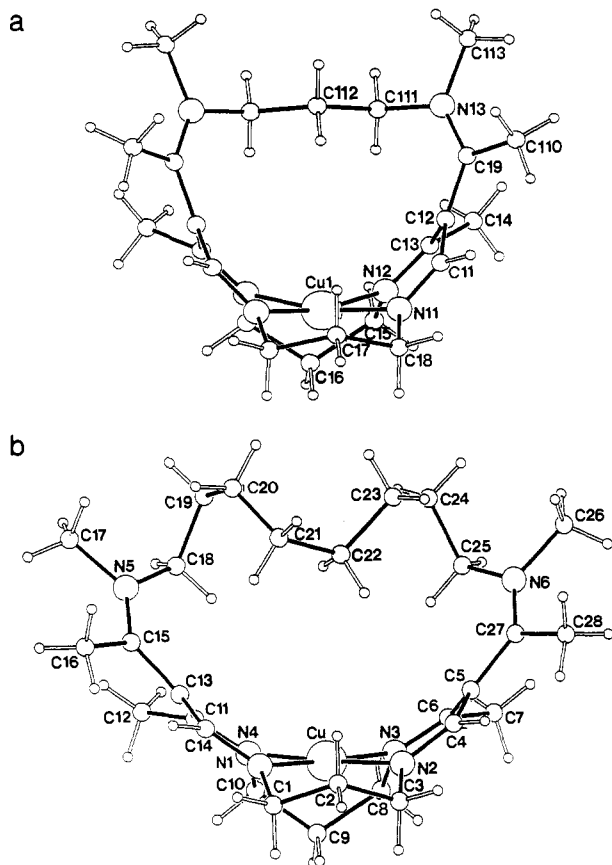
Figure 7. Narrow and wide polymethylene-bridged cyclidene complexes: (a) \text{Cu}^{\text{II}}(\text{C3MeMe}[16]\text{Cyc}) and (b) \text{Cu}^{\text{II}}(\text{C8MeMe}[16]\text{Cyc}) .
