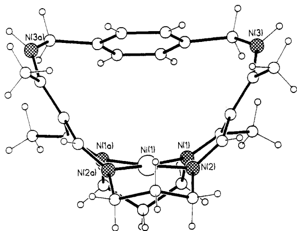
Figure 9. A p -xylylene-bridged cyclidene, Ni II ( p XyHMe[16]Cyc).
