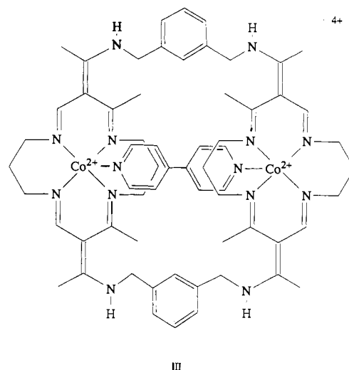
Figure 32. Coordinated 4,4'-bipyridine guest in cavity of ditopic dicobalt cyclidene.
